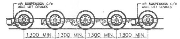
OPTIONAL RUNNING GEAR ARRANGEMENT
